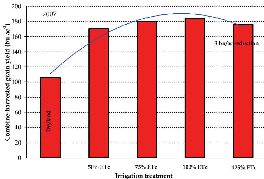
Figure 1. Corn yield response to different levels of irrigation, including an over-irrigated plot (irrigations were replenished at 125 percent of the actual crop water use rate, evapotranspiration) at the University of Nebraska–Lincoln, South Central Agricultural Laboratory near Clay Center, Neb. Plots were irrigated using a subsurface drip irrigation system.
