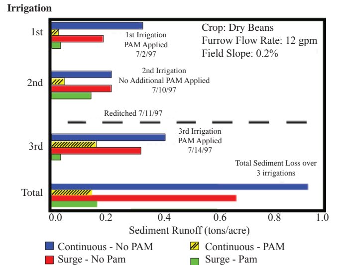
Figure 4. 1997 Sediment Loss (tons/acre) for each irrigation and total sediment loss (tons/acre) for treatments of no PAM continuous irrigation, PAM continuous irrigation, no PAM surge irrigation and PAM surge irrigation.
