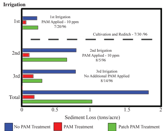
Figure 2. 1996 Sediment Loss (tons/acre) for each irrigation and total sediment loss (tons/acre) for treatments of no PAM, PAM, and patch PAM.
