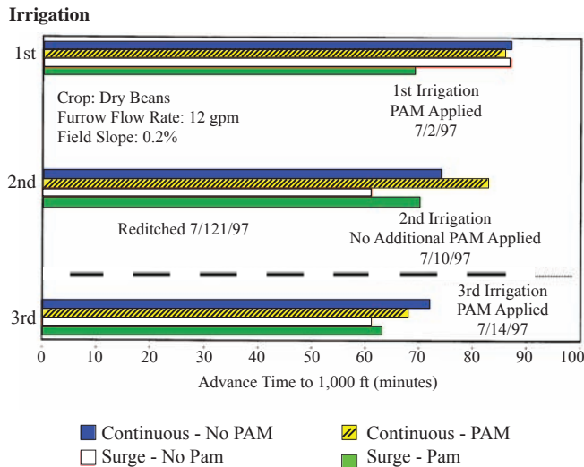
Figure 3. 1997 Furrow advance time to 1,000 feet for each irrigation, treatments of no PAM continuous irrigation, PAM continuous irrigation, no PAM surge irrigation and PAM surge irrigation.
