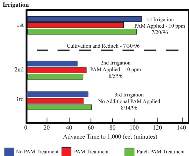
Figure 1. 1996 Furrow advance time to 1,000 feet for each irrigation, treatments of no PAM, PAM, and patch PAM.
