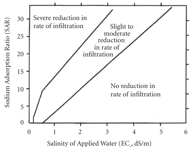
Figure 3. Relative rate of water infiltration as affected by salinity and sodium adsorption ratio.
