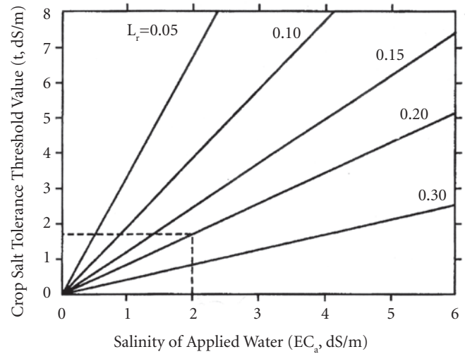
Figure 4. Leaching requirement ( L_r ) as a function of the salinity of the applied water and the crop's salt-tolerance threshold value.
