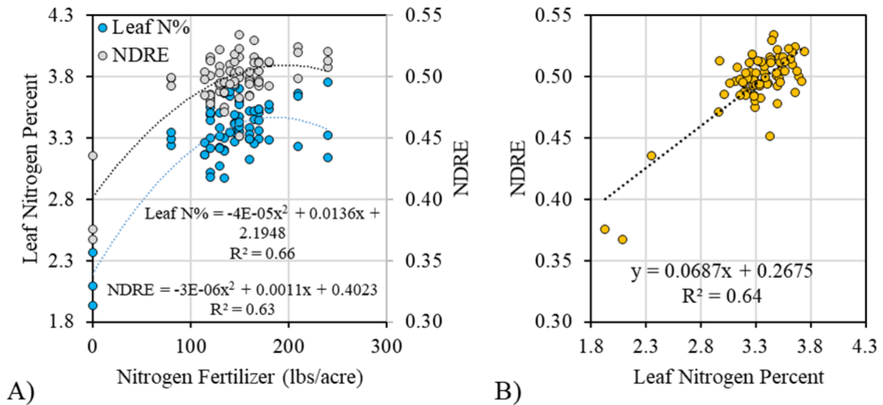
Figure 13. On July 18, leaf tissue samples were collected for percent nitrogen (N) and normalized difference red edge (NDRE) was calculated using canopy reflectance measured from four crop circles (Holland Scientific Inc., Lincoln, NE, USA). Leaf N percent and NDRE as compared with applied N fertilizer (A) and NDRE as compared with leaf N percent (B).
